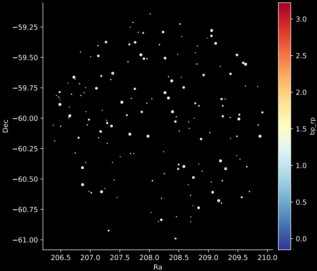
APOGEE DR17 Field: [271-21-O_TESS] Stars: 157
