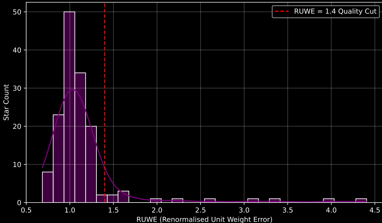
GAPOGEE DR17 Field [271-21-O_TESS] RUWE Distribution (n= 149)
