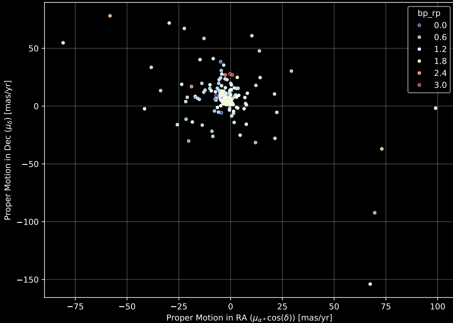
APOGEE DR17 Field: [271-21-O_TESS] Proper Motion Diagram (n= 157)
