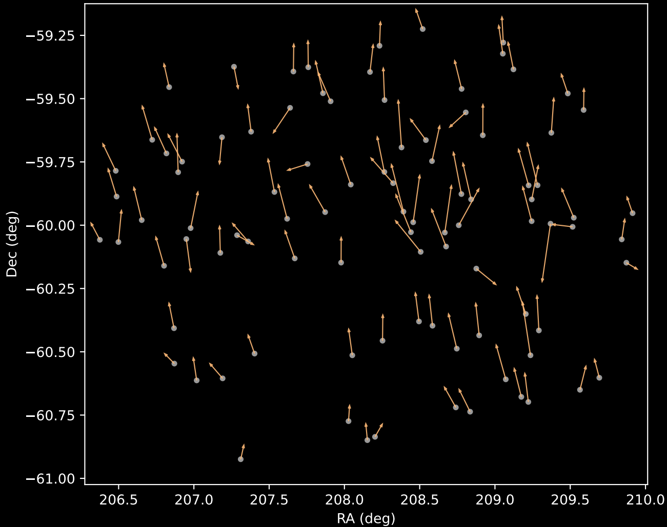
APOGEE DR17 Cluster 3 Proper Motion Vectors (n=94)
