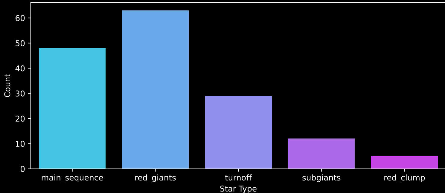
APOGEE DR17 Field: [271-21-O_TESS] Count plot of Star Type
