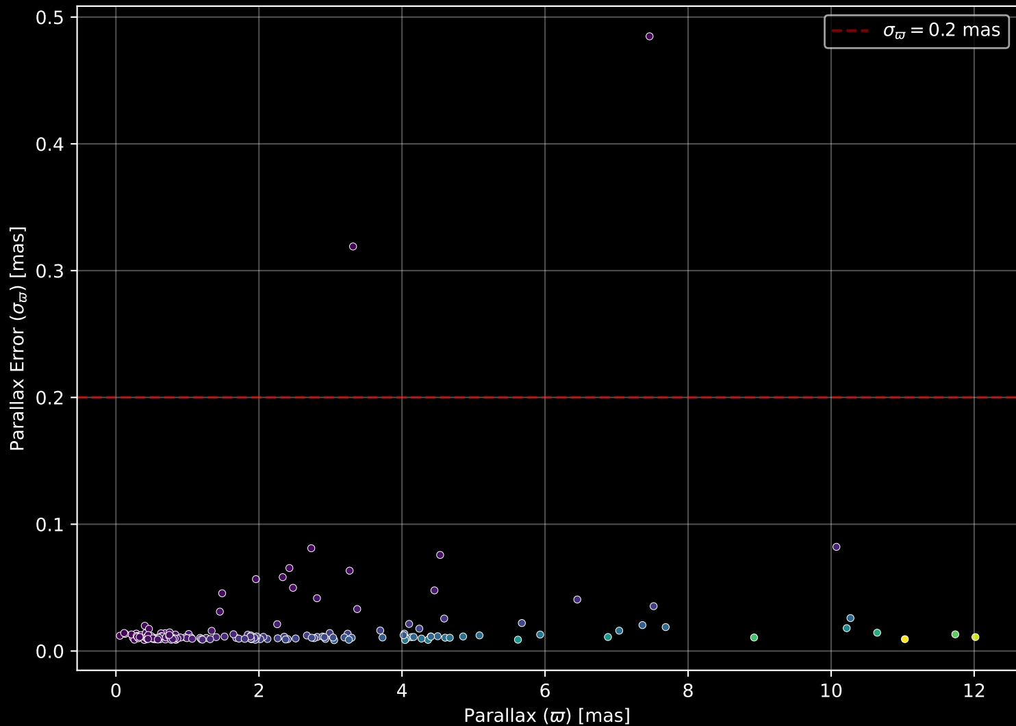
APOGEE DR17 Field: [271-21-O_TESS] Parallax Quality (n= 157)
