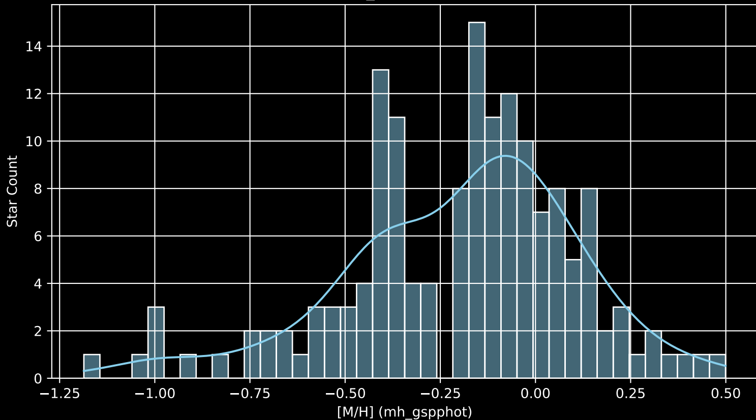
APOGEE DR17 Field: [271-21-O_TESS [M/H] (mh_gspphot) (n= 155)
