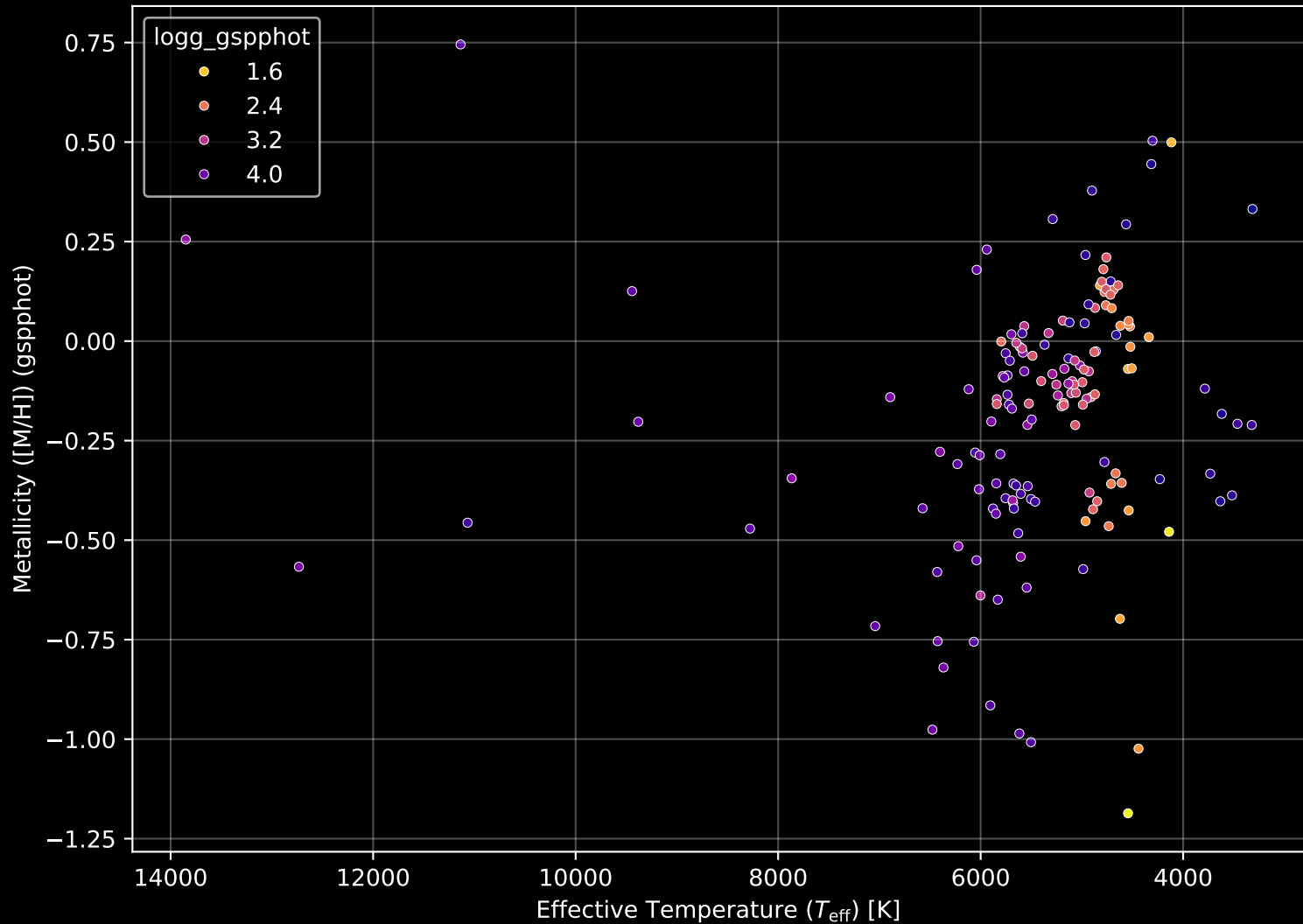
APOGEE DR17 Field: [271-21-O_TESS] Stellar Population Parameters (n= 157)
